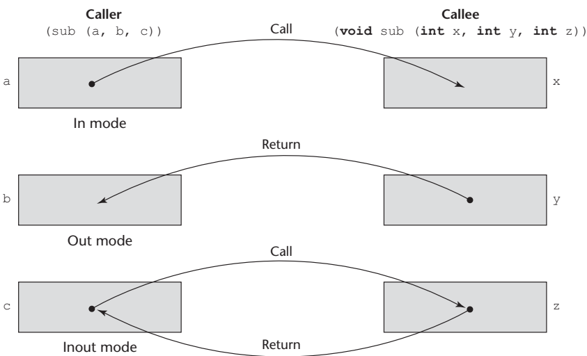
Figure 9.1 The three semantics models of parameter passing when physical moves are used
